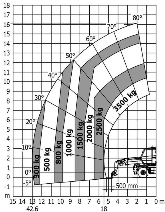
フォークFloating Fork Carriage (TFF4T)Ref.924857
