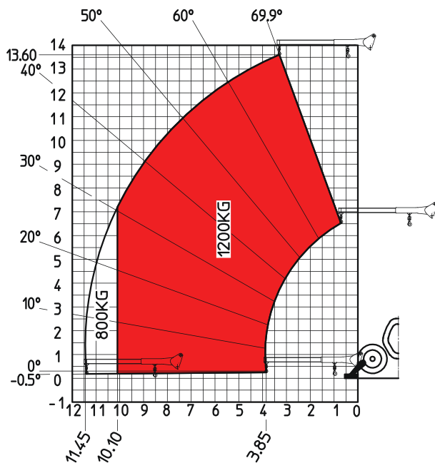
Machine on stabilizers with 2-hook jib P 4000
