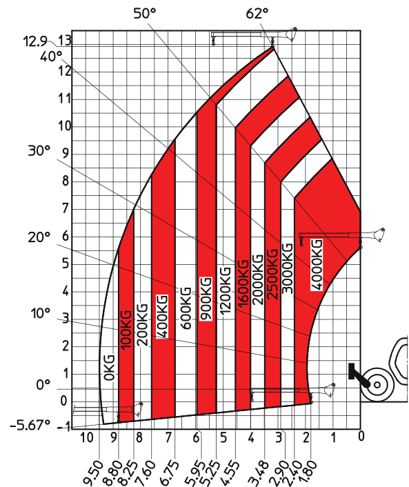
Machine on tyres with 2-hook jib P 4000
