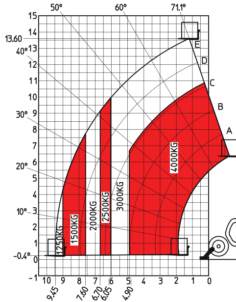
Machine on stabilizers with forks
