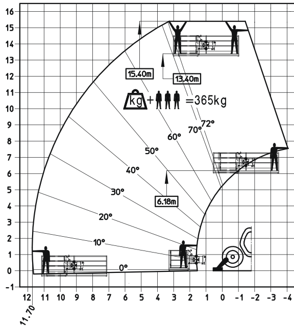
Machine on stabilizers with PSE 4400 / 365 D platform
