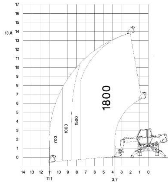
Rotation on stabilizers with 1m 3 bucket CBR1000
