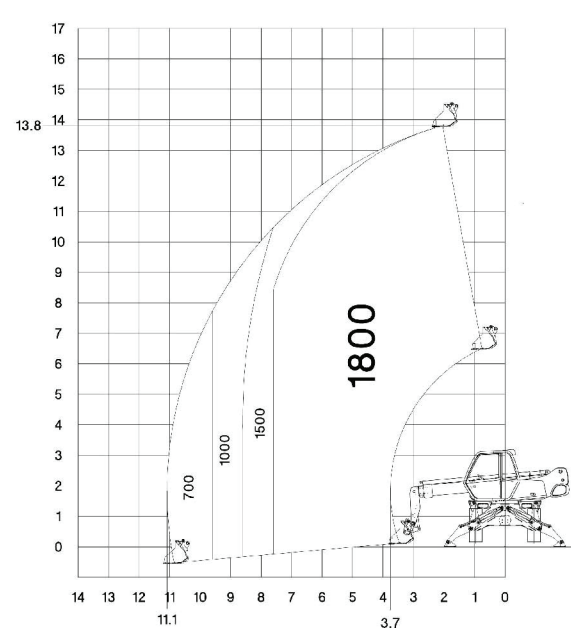
Rotation on stabilizers with 1m³ bucket CBR1000
